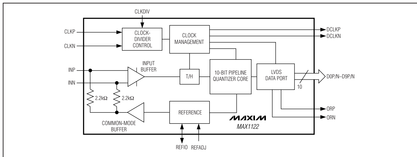
Figure 1. MAX1122 Block Diagram
